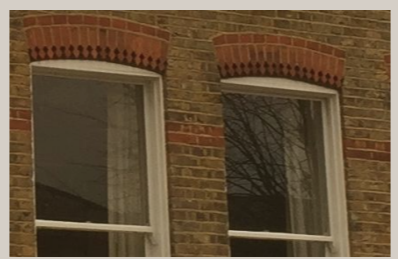
Special brick flat arch over sash windows
